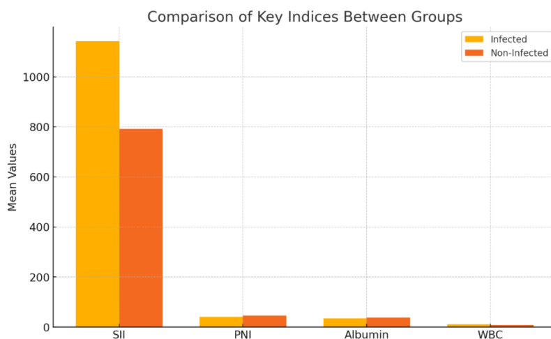
Figure 2. Comparison between infected and non-infected groups. PNI: prognostic nutritional index; SD: standard deviation; SII: systemic immune-inflammation index; WBC: white blood cell.
