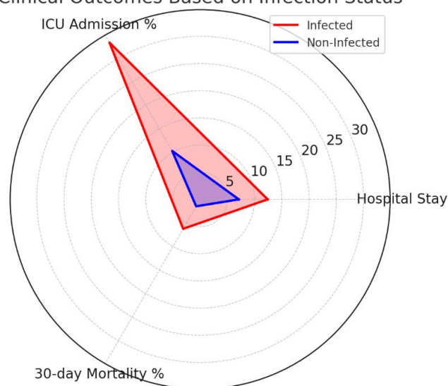
Figure 3. Clinical outcomes according to infection status. ICU: intensive care unit.
