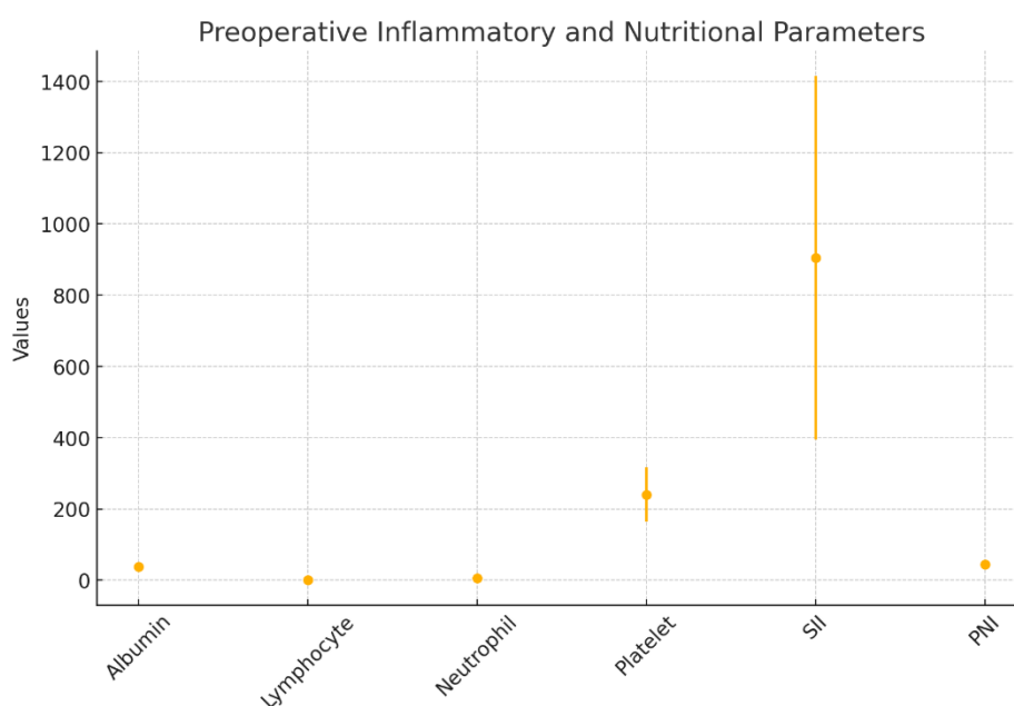
Figure 1. Preoperative inflammatory and nutritional parameters. PNI: prognostic nutritional index; SD: standard deviation; SII: systemic immune-inflammation index.
