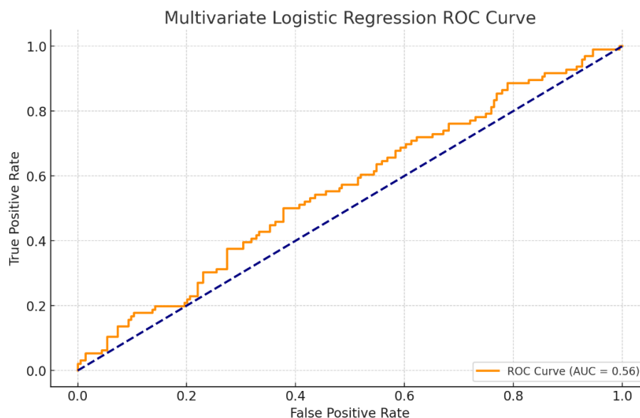
Figure 4. Multivariate logistic regression for predicting infection. CI: confidence interval; OR: odds ratio; PNI: prognostic nutritional index; SII: systemic immune-inflammation index.
