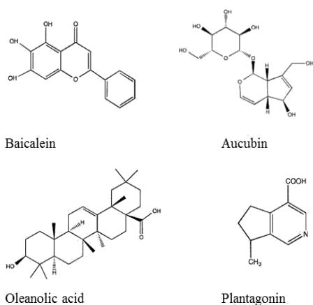
Figure 1. Some chemical structural of Plantago major ( P. Major ) compounds including baicalein (flavonoid), aucubin (irioid glycoside), oleanolic acid (terpenoid) and plantagonin (alkaloid)
